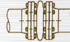
Axial Compression
