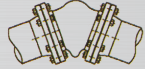
Angular Deflection
