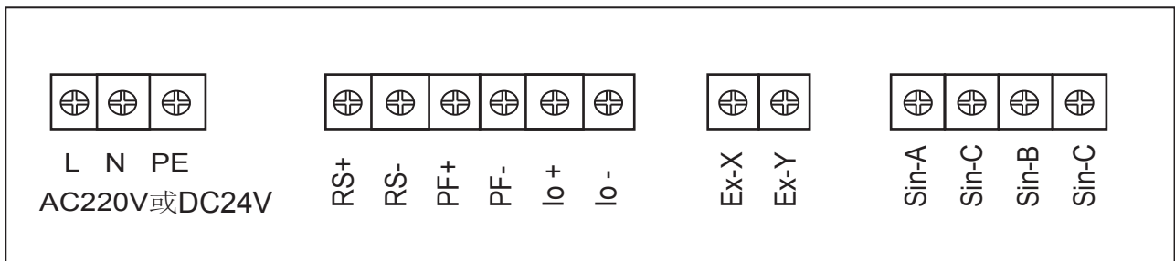
Diagram of output signal terminal Terminal Description
