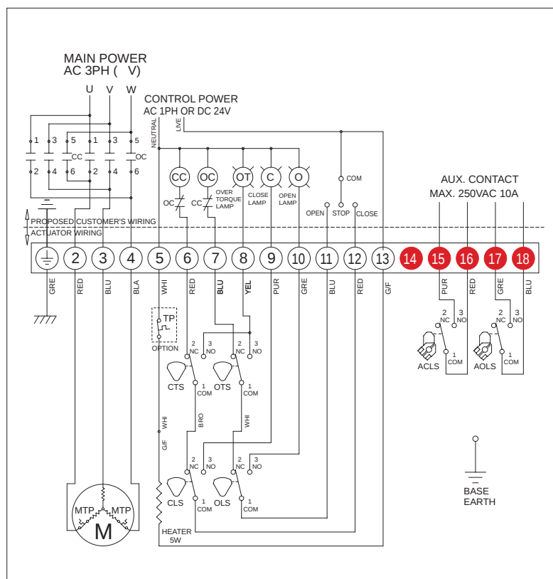
380/440VAC/50/60Hz, 3Ph(On-Off)
