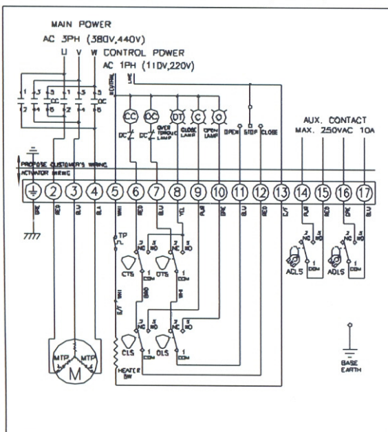
ATM0160~3000(3Ph)
