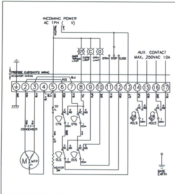
ATM0160~3000
