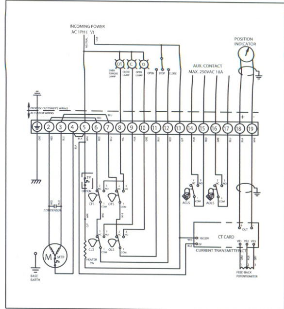
ATM0160~3000(CT CARD)
