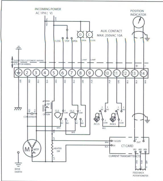
ATM0100(CT CARD)
