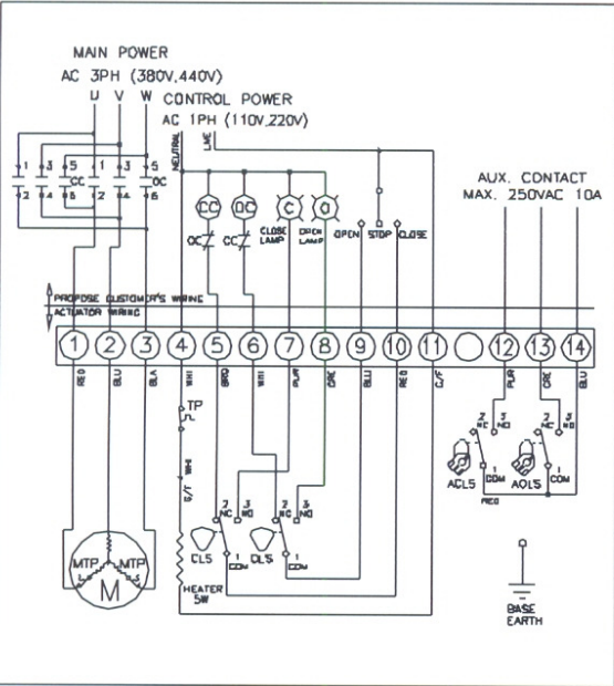
ATM0100(3Ph)
