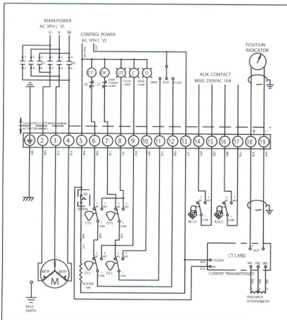
ATM0160~3000(CT CARD)
