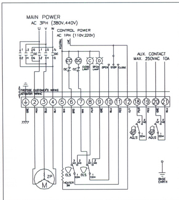
ATM0080(3Ph)
