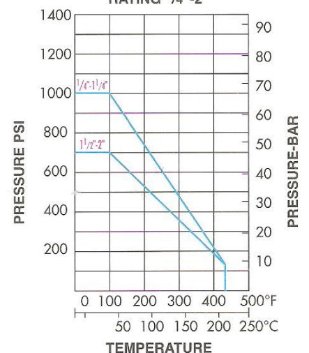
PRESSURE-TEMPERATURE RATING 1/4"-2"
