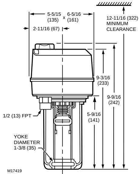
Fig. 1. Approximate dimensions of ML6420, ML7420 Electric Linear Valve Actuator in in. (mm).
